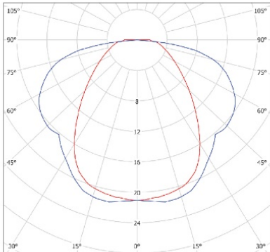
Light Distribution Curve
